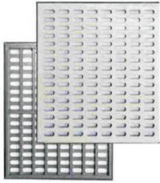
◆ 36% rate air-flow
